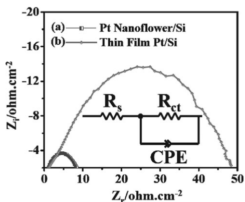
Fig. 4 Nyquist plot of electrochemical impedance spectra (EIS) of the 3D Pt nanoflowers and the Pt thin film catalysts in 1 M \text{CH}_3\text{OH} –1 M \text{H}_2\text{SO}_4 solution at the potential of 0.3 V. The inset shows the equivalent circuit model used to fit the impedance spectra.
